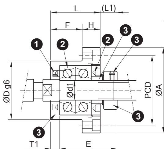
Installation A
