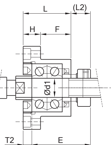
Installation B
